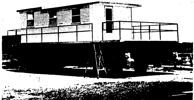
READY FOR LAUNCHING. This houseboat was built over the past six months by Paul, Karl, Heinz and Kurt Otto and Wes Beckenhauer at the rear of the Otto Construction Co. offices a mile east of Wayne. The boat is 14 by 36 feet long and is powered by twin 40 horsepower in-board-outboard motors. The cabin is 10 by 22 feet long and has booths which make into sleeping beds. The 10,000 pound boat was launched at Weigand on the Lewis and Clark Lake recently.
